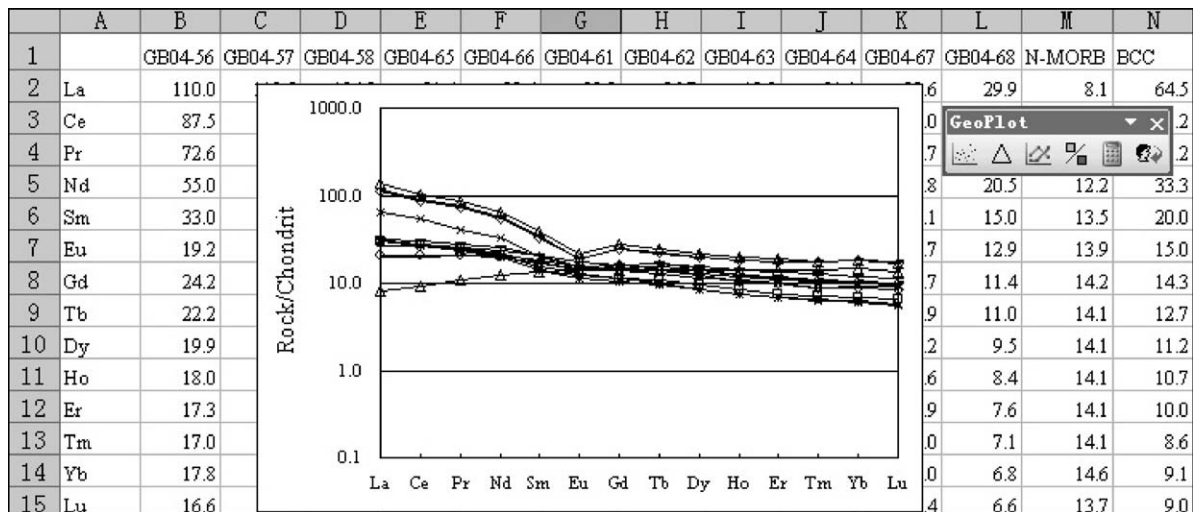
Fig. 4. Chondrite-normalized data and resultant REE distribution diagram.
